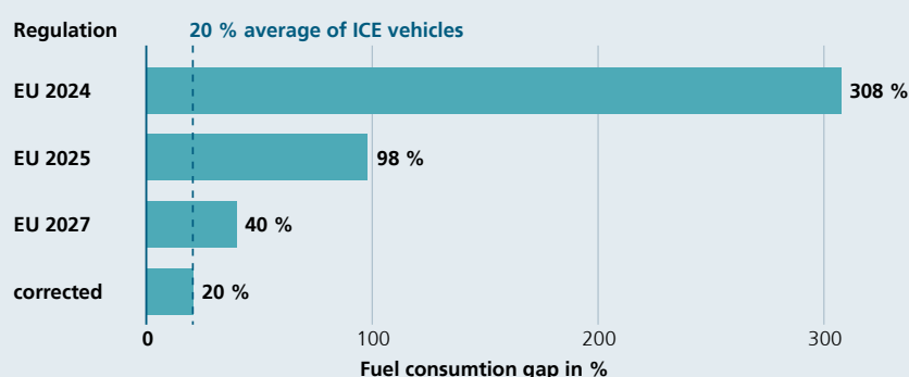
Figure 2: Percentage gap between nominal and real-world fuel consumption of PHEVs in Europe according to different regulations
