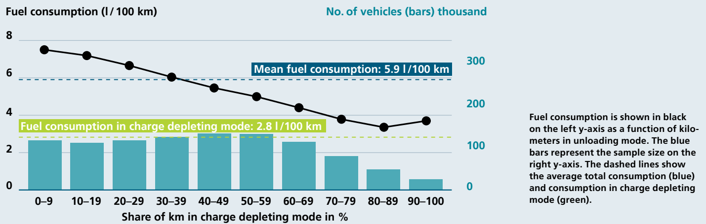
Figure 1: Actual fuel consumption as a function of CD mode share.
